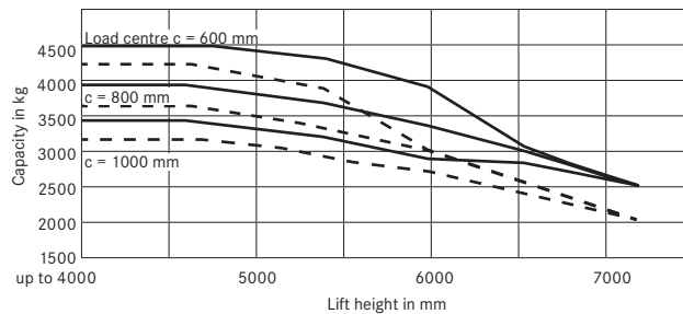
Capacities RX 60-45/600 with triplex mast
