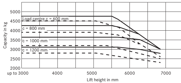
Capacities RX 60-50/600 Triple mast from BH2400
